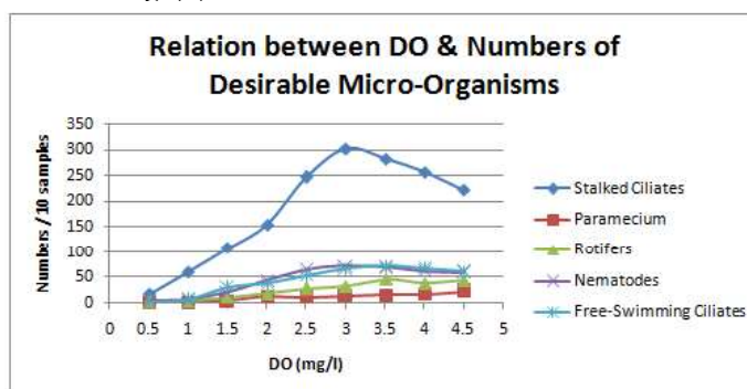
FIG 4. Numbers of desirable micro-organisms (Stalked Ciliates, Paramecium, Rotifers, Nematodes and Free Swimming Ciliates) in the pilot plant and relation between micro-organisms and dissolved oxygen (DO)
