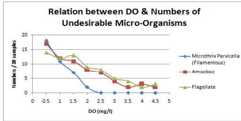
FIG 5. Numbers of undesirable micro-organisms (Microthrix Parvicella, Amoeba and Flagellate) in the pilot plant and relation between micro-organisms and dissolved oxygen (DO)
