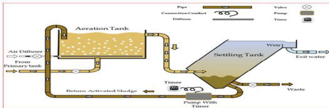
FIG 2. Schematic diagram of the pilot plant
