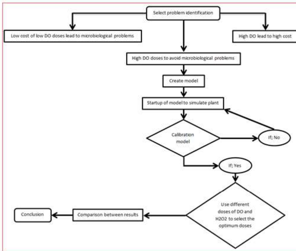
FIG 3.The Work Program Flow Chart
