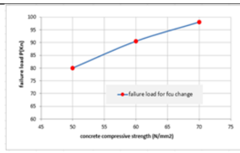
Fig 16: The relationship between concrete compressive strength and the residual capacity
