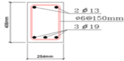
(b) Cross- section
