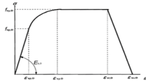
Fig 1: Mathematical model for stress strain curve for uniaxial compression at elevated temperature [11]
