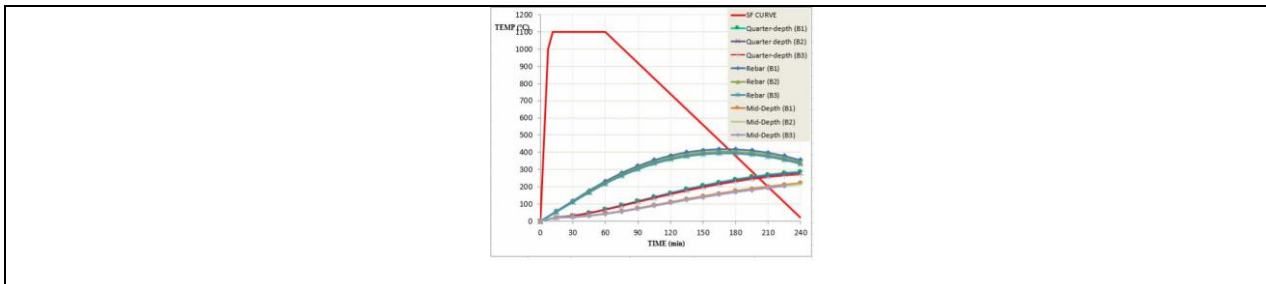
Fig 14 : Temperature distribution at various elevated temperatures at different positions for beams B1, B2 and B3
