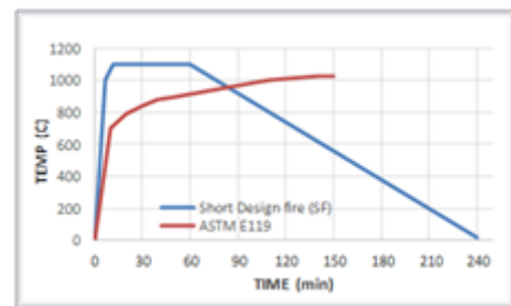
Fig 5: ASTM E119 and short fire curve (SF)
