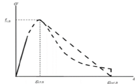
Fig 2: Mathematical model for both reinforcing steel and pre-stressing steel at elevated temperatures [11]
