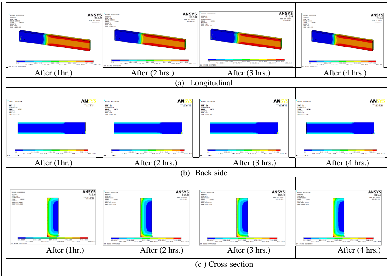
Fig 13 : Thermal contours for beam B1 after 1hr., 2 hrs., 3 hrs. and 4 hrs
