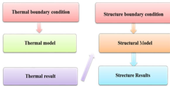
Fig 3: Sequential coupling technique
