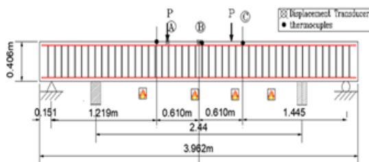
(a) Longitudinal view
